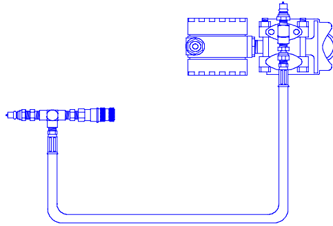
Casing Pressure (Choke Line)
